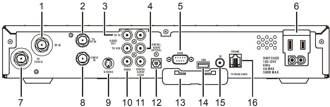
Figure 2-2 Rear panel
